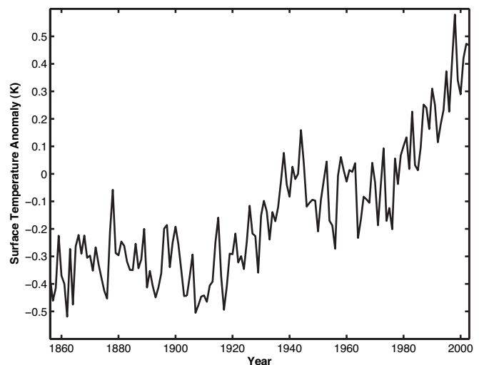
Fig. 1. The annual GSTA from 1856 to 2003.
